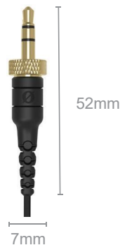
TRS CONNECTOR
