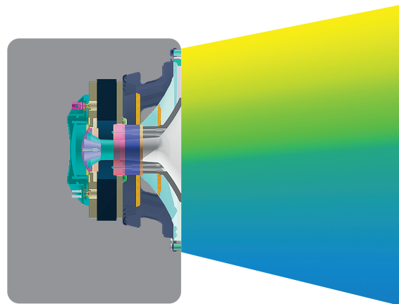
Horn loaded Coaxial Dispersion
